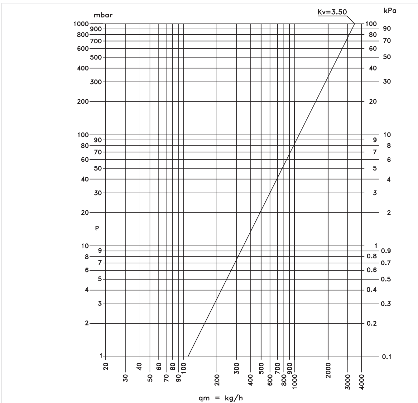
Diagram of load losses of deviator valve, present in kit EK3VK1 in completely open position.
